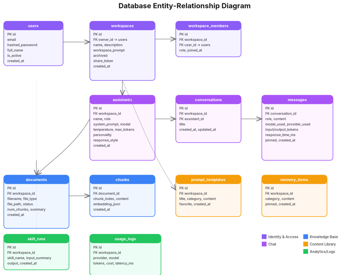
Figure 1. Database Entity-Relationship Diagram
